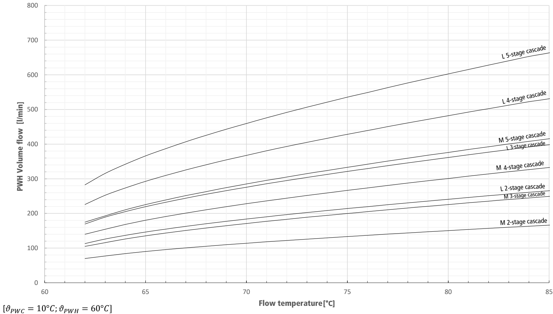
Performance Diagram PWH 60 °C
