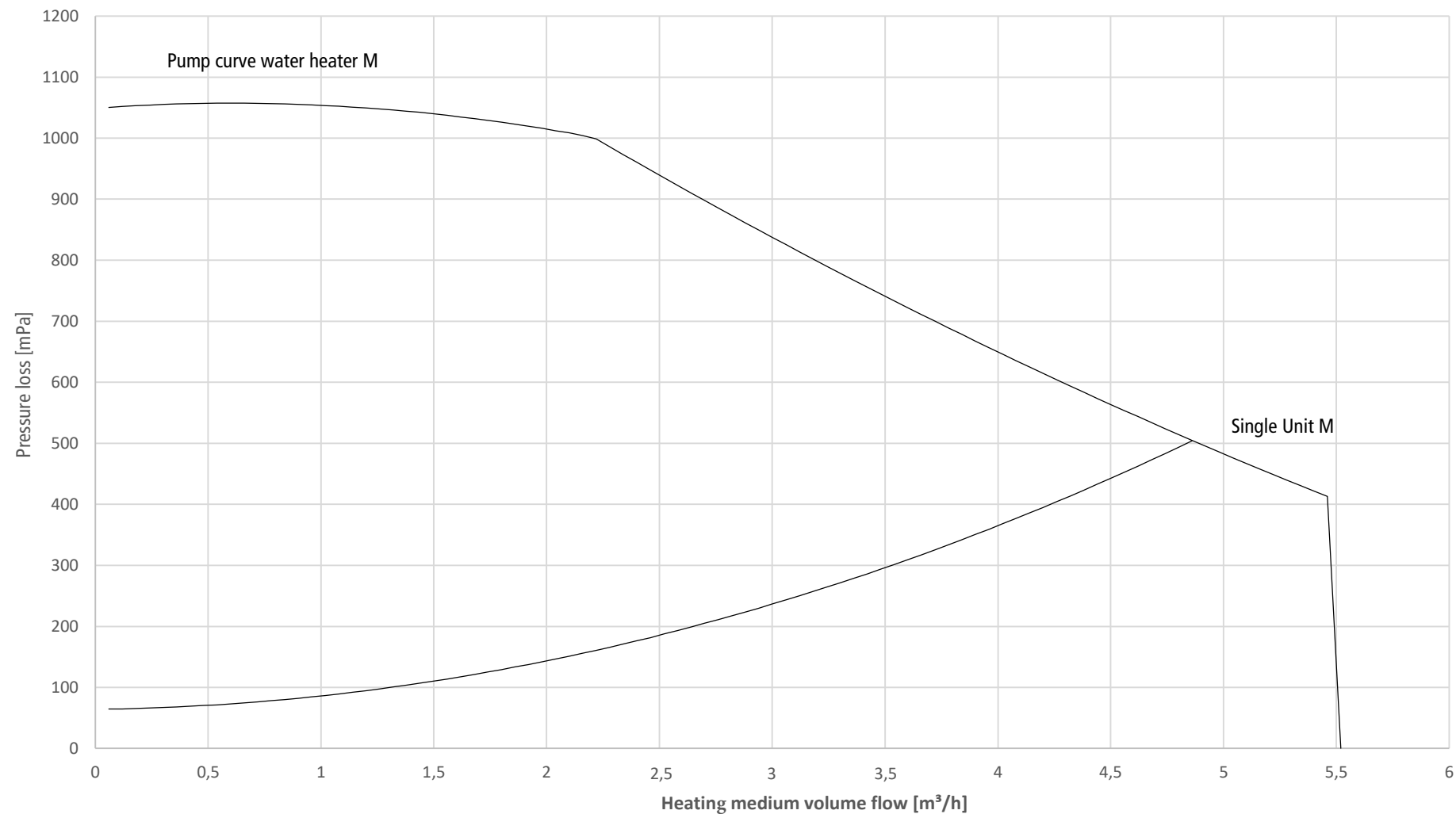
Pump Curve and Primary Pressure Loss M
