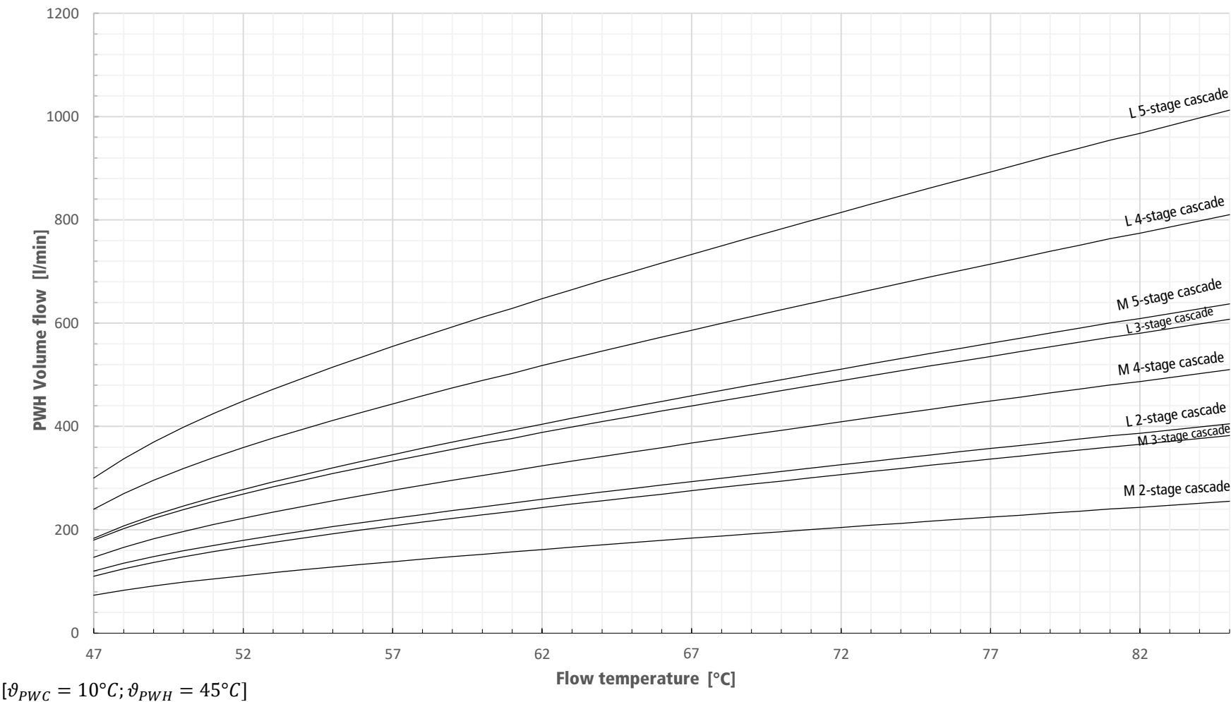
Performance Diagram PWH 45 °C
