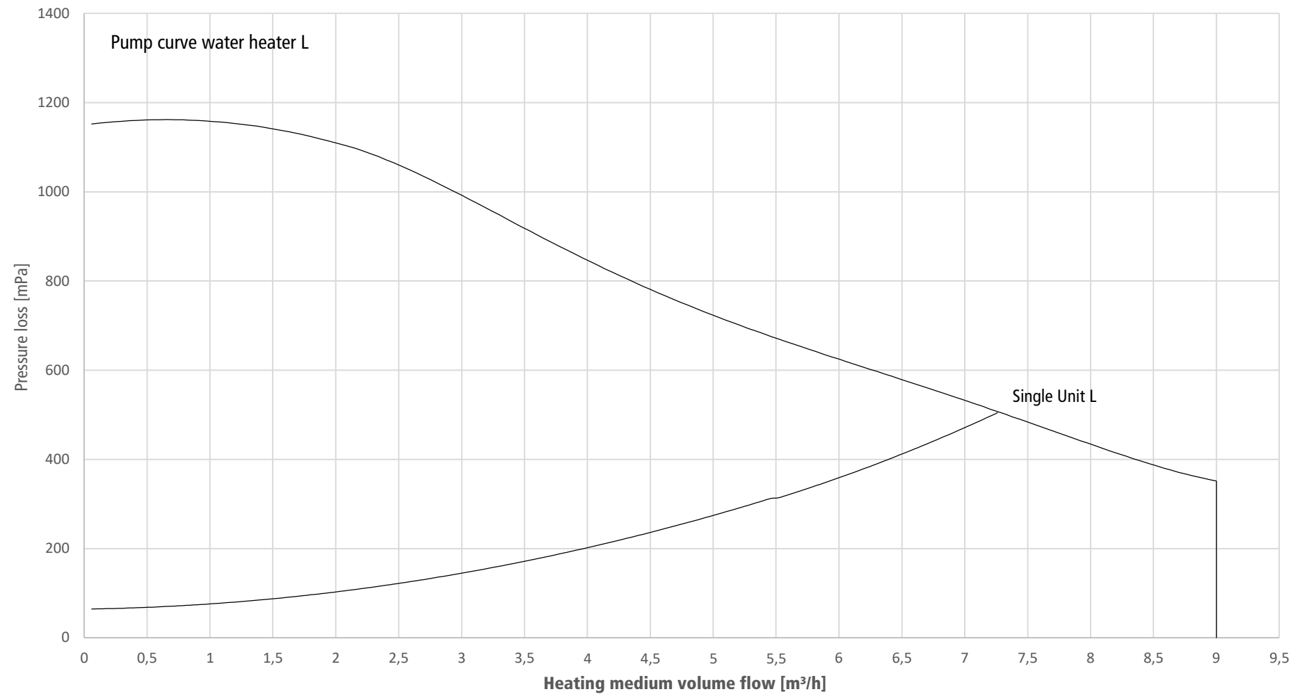
Pump Curve and Primary Pressure Loss L
