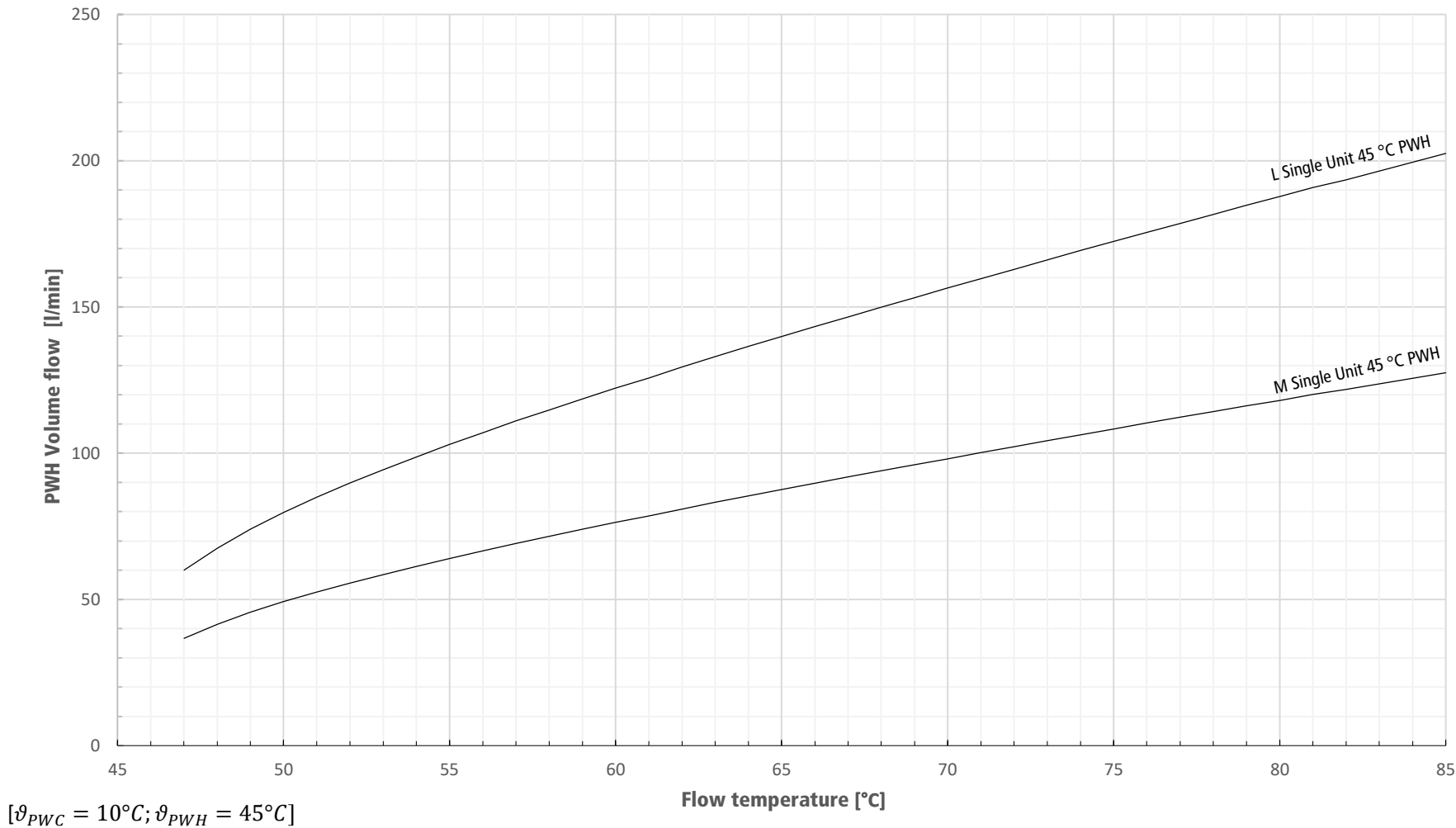
Performance Diagram Single Units PWH 45 °C
