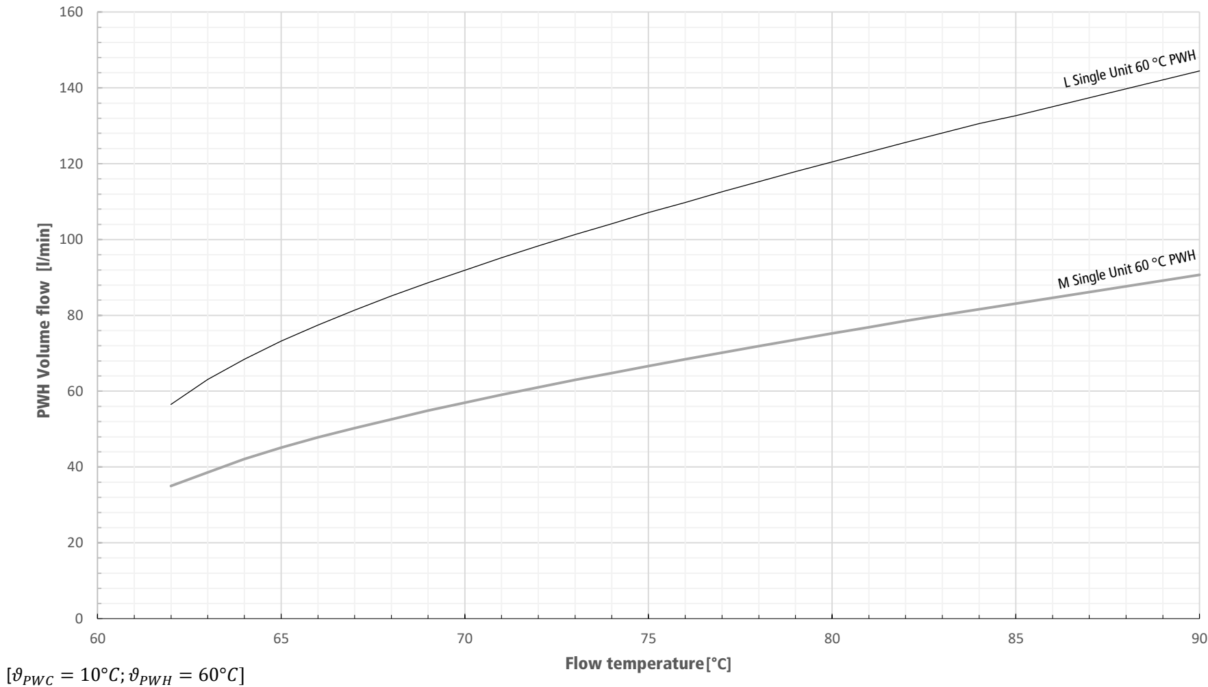
Performance Diagram Single Units PWH 60 °C
