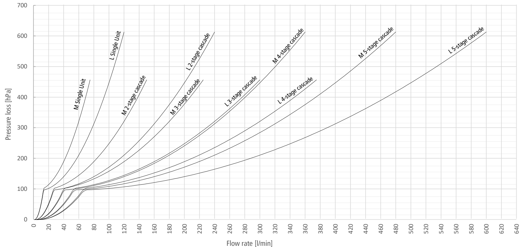
Pressure Loss Drinking Water Side (Secondary)
