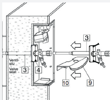
Exposed installation
