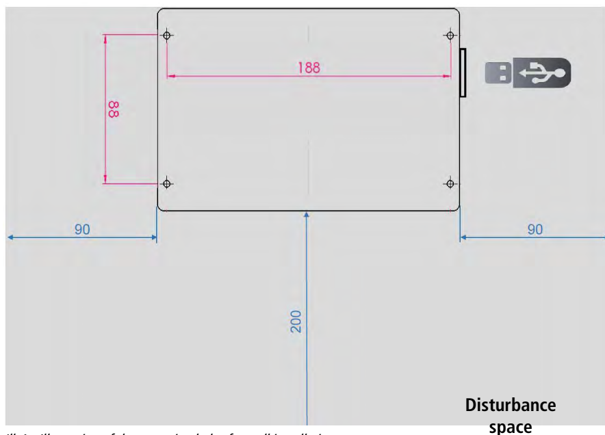
III. 1 - Illustration of the mounting holes for wall installation
